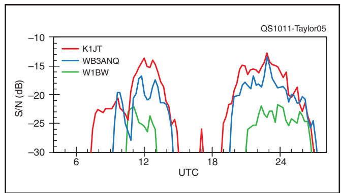
Figure 5 — Average S/N reported by VK6DI (Western Australia) for K1JT, WB3ANQ and W1BW (all in northeast USA) during March and April 2009 on the 30 meter band, plotted vs time of day.
